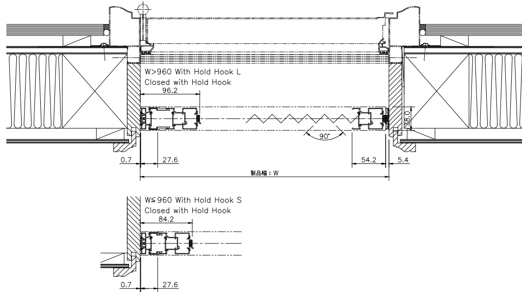
Zipooh Single door (8LME) Cross section
