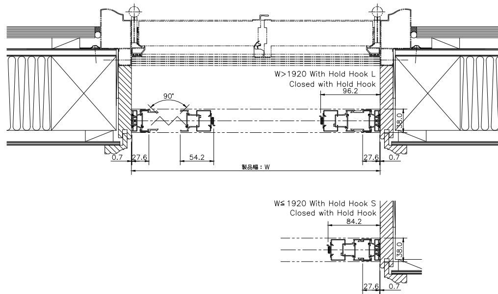
Zipooh Double door (8LME) Cross section
